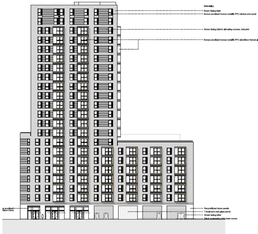
Elevation 4 – Proposed North East Elevation (Source: Applicant)
